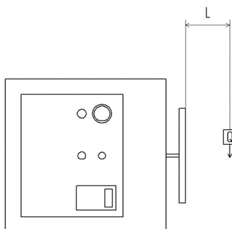
Horizontal Load
