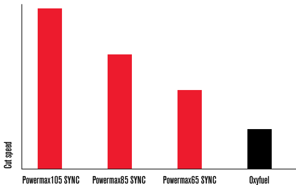
Relative cut performance on 12 mm (1/2") mild steel
